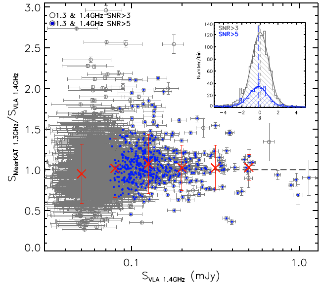
Figure 1. Ratio of ‘superdeblended’ flux densities at MeerKAT 1.3 GHz and VLA 1.4 GHz as a function of 1.4 GHz flux density for the 1599 sources with SNR > 3 at both frequencies. We mark the sources that have SNR > 5 at both frequencies by blue solid points. The red crosses are the median ( S_{1.3}/S_{1.4} ) for sources within each 1.4 GHz flux density bin. The inset plot shows the distribution of normalized difference of ‘superdeblended’ flux densities at these two frequencies for sources with SNR > 3 and SNR > 5 at both frequencies, respectively. Overall, despite the scatter, the ‘superdeblended’ flux densities extracted from the VLA 1.4 GHz and MeerKAT 1.3 GHz data are consistent with each other within the uncertainties for sources with SNR > 5 if we consider their slightly different effective frequencies.
