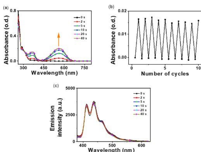
Figure 6. (a) Absorption spectra of 2 in toluene solution ( 2 \times 10^{-5} M) upon UV-light irradiation ( 0.96 \text{ mW/cm}^2 ), (b) photo-switching cycles of the absorbance at \lambda_{\text{max}} (562 nm) of 2 upon alternating 302 nm UV-light ( 0.96 \text{ mW/cm}^2 ) and 621 nm visible-light ( 21.5 \text{ mW/cm}^2 ) irradiations, (c) emission spectra of 2 upon UV-light irradiation ( 0.96 \text{ mW/cm}^2 ), concentration = 2.5 \times 10^{-6} M.
