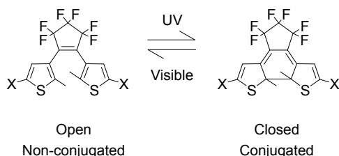
Figure 1. Photochromism of dithienylethene (DTE) derivatives.
