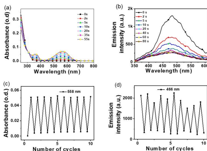
Figure 5. (a) UV-Vis absorption spectra and (b) emission spectra of 2 in PMMA film upon 302 nm UV-light irradiation (0.96 mW/cm 2 ), showing the open-form to closed-form transition, at different time intervals, excitation wavelength = 320 nm. The photoswitching cycles of the (c) absorption and (d) fluorescence at maximum wavelength upon alternating UV-light (1.83 mW/cm 2 , 302 nm) and visible-light (21.5 mW/cm 2 , 621 nm) irradiations. Concentration = 5 wt% in PMMA.
