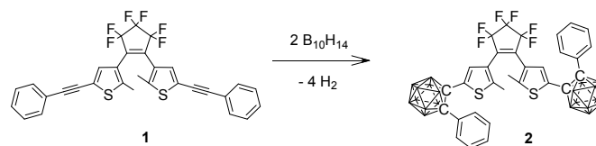
Figure 2. DTE derivatives 1 and 2 discussed in this work. Each unlabelled vertex in the clusters is BH.
