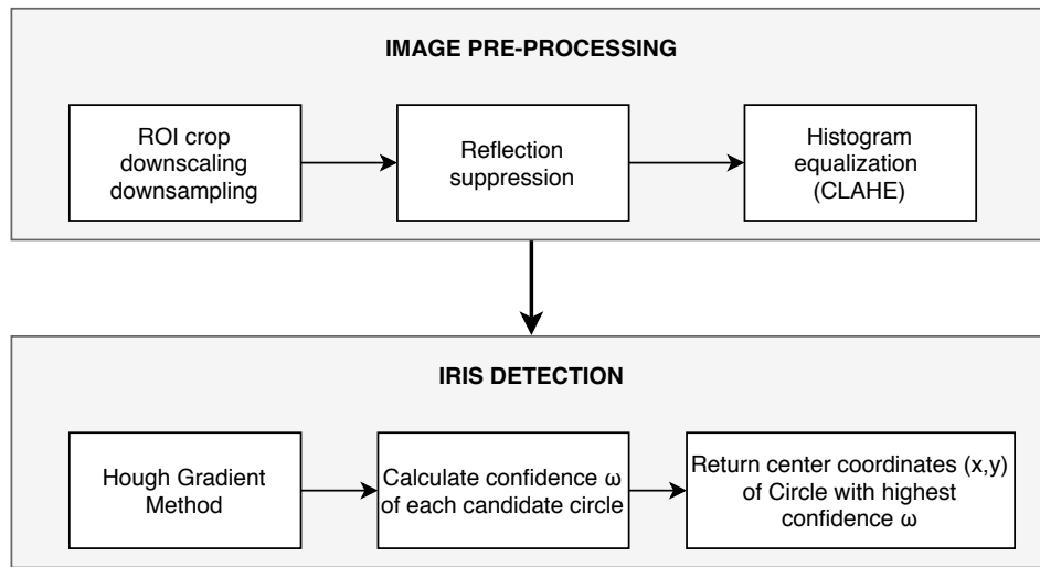
Fig. 3. Flowchart depicting the steps involved in processing the original image to calculate the iris center position.
