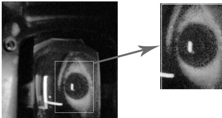
Fig. 4. ROI detection provides as input to the next process a subsection of the captured images, representing the detected ROI rectangle. Two strong reflections are also visible - one on the headset's lens and one on the cornea.
