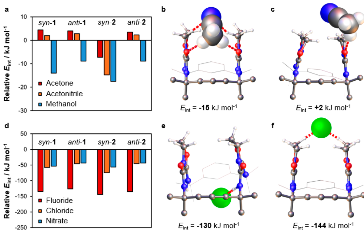
Figure 15. (a) Calculated (B3LYP/6-31++G**) interaction energies ( E int ) for complexes of 1 and 2 with neutral guests and the most stable binding complexes of acetonitrile with (b) 2 and (c) 1 . (d) E int values for complexes of 1 and 2 with anionic guests and the most stable (e) NH...F - and (f) CH...F - contacts in fluoride complexes of 2 . All E int values are expressed relative to the corresponding chloroform complexes. Hydrogen bonds and major dipole–dipole interactions are marked in red, and parts of the macrocycles are omitted for clarity.
