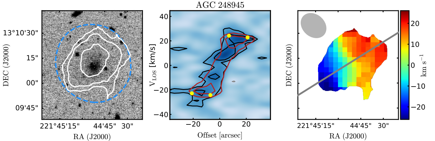
Figure 1. A representative galaxy from our sample, AGC 248945. Left: H I contours on top of the r -band image; the contours are at 0.88, 1.76 and 3.52 \times 10^{20} H I atoms per \text{cm}^2 , the outermost contour corresponds to \text{S/N} \approx 3 . The blue ellipse shows the inclination the galaxy would need to be in the BTFR (see the text for details). Middle: PV-diagram along the kinematic major axis; black and red contours correspond to data and 3^{\text{D}} Barolo best-fit model, respectively; the yellow points show the recovered rotation velocities. Right: Observed velocity field, at the same scale as the left panel. The grey line shows the kinematic major axis and the grey ellipse the beam.
