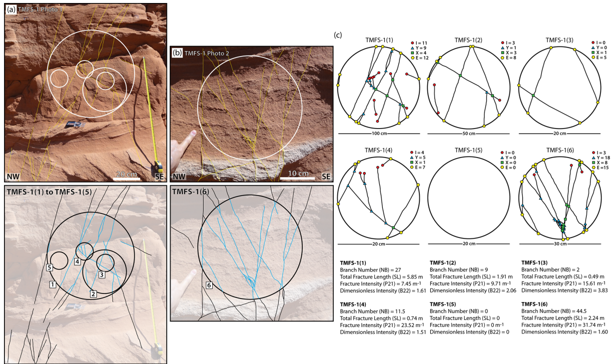
Figure A1. Sample station TMFS-1 scan circles (a, b) and nodal analysis (c) with statistics.
