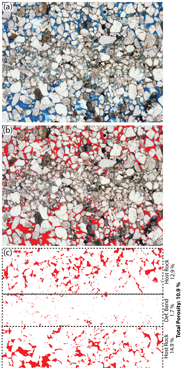
Figure 6. Quantitative determination of porosity percentages using ImageJ. (a) Sections were impregnated with blue-dyed plastic resin in order to highlight porosity. (b) Image analysis using ImageJ to select areas (red) containing blue dye. (c) Percentage areas (porosities) can then be calculated for both whole section and selected areas (e.g. host rock vs deformation band). Note the substantially lower porosity and smaller pore size within the deformation band.
