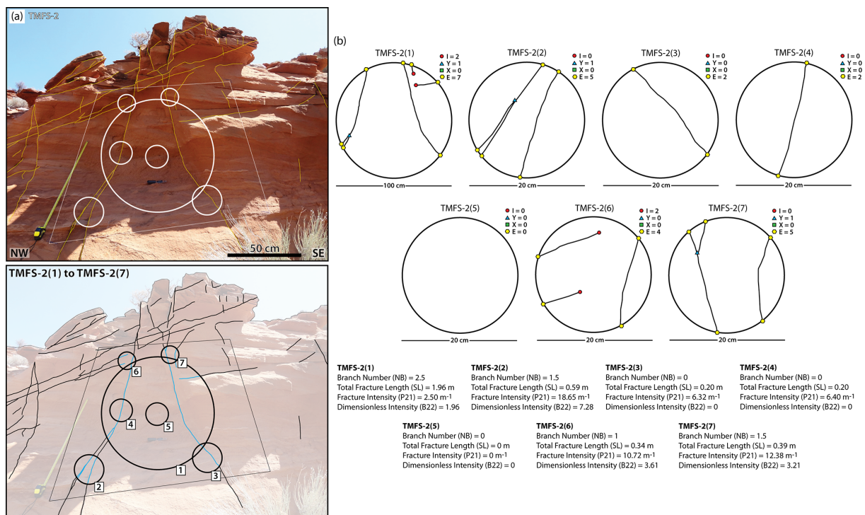
Figure A2. Sample station TMFS-2 scan circles (a) and nodal analysis (b) with statistics.
