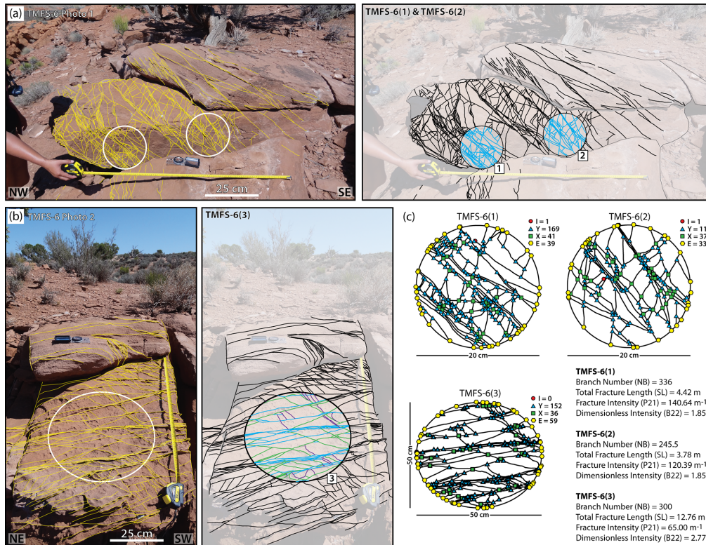
Figure A6. Sample station TMFS-6 scan circles (a, b) and nodal analysis (c) with statistics.
