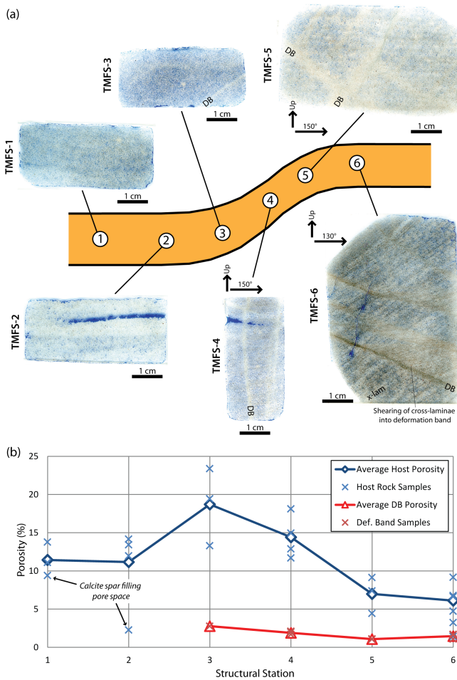
Figure 8. Porosity variability across the intrusion margin. (a) Whole thin-section photographs (flatbed scans) for each structural station. Blue dye denotes porosity in each sample. (b) Plot showing variability in porosity observed in this study for each station. Porosity percentages were calculate using the image analysis software package ImageJ as shown in Fig. 6. Note, a similar porosity reduction trend has been observed previously (see Fig. 8 in Morgan et al., 2008). DB: Deformation Band; X-lam: Cross-lamination.
