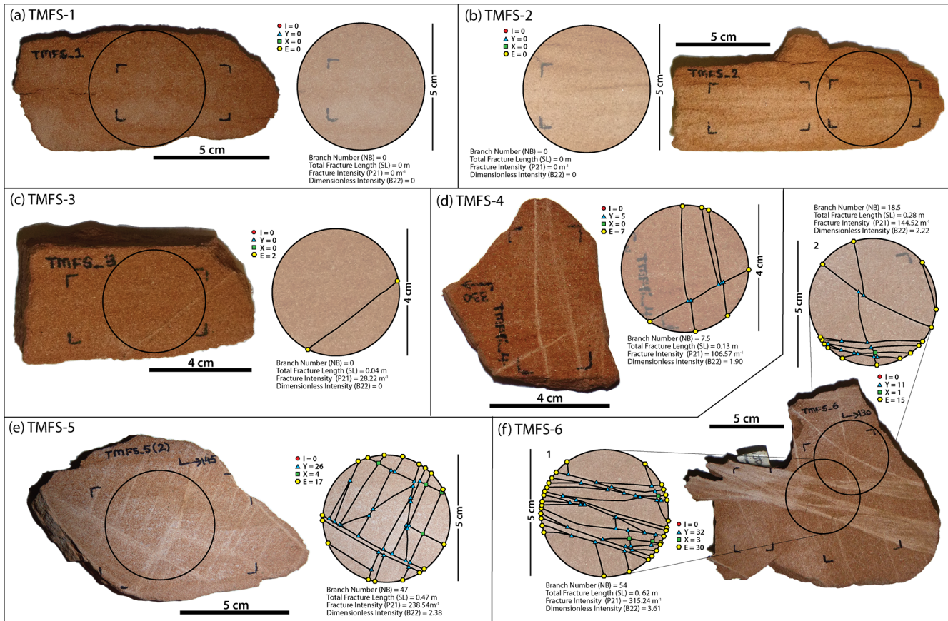
Figure 3. Fracture analysis of hand specimens. (a–f) Bedding-normal cut surfaces with hand-specimen photographs showing fracture analysis circles for each structural station (note, sample numbers correspond to their respective station). Fracture analysis was carried out on freshly cut surfaces. Circular scans show the fracture network and associated I-, Y-, X- and E-nodes (for explanation of terminology see Fig. 4 and Sanderson and Nixon, 2015). Statistics show total number of branches ( N ), total fracture length (SL), fracture density/intensity ( P_{21} ), and branch dimensionless intensity ( B_{22} ).
