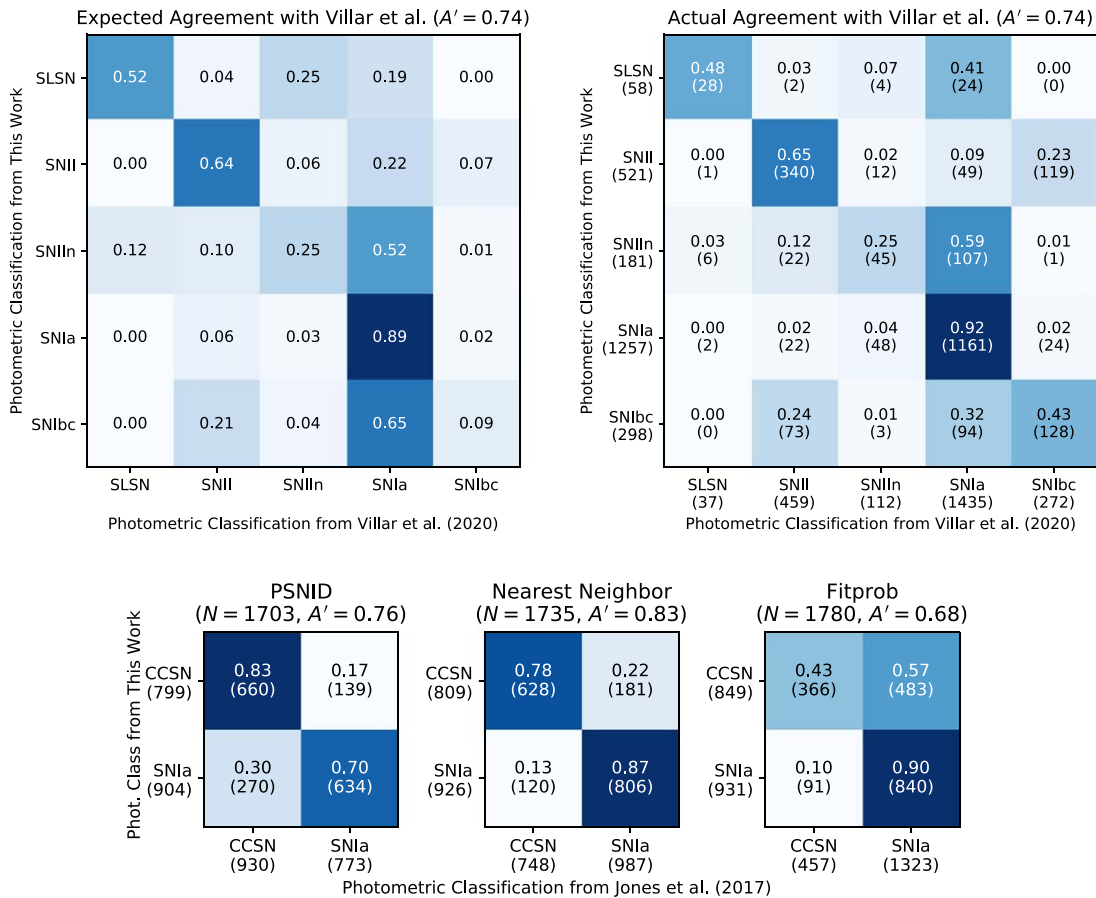
Figure 10. Top left: expected agreement between our classifier and that of V20 , given our confusion matrices from validation (see Appendix B). We expect very low agreement on SNe IIn and Ibc, which both classifiers independently struggle with. Top right: actual agreement with V20 . As expected, we agree on A' = 74\% of classifications overall, including a larger than expected fraction of SNe Ibc (43%). Bottom: agreement between our classifier and those of Jones et al. (2017) , where all classes that are not SNe Ia are aggregated under the CCSN label.
