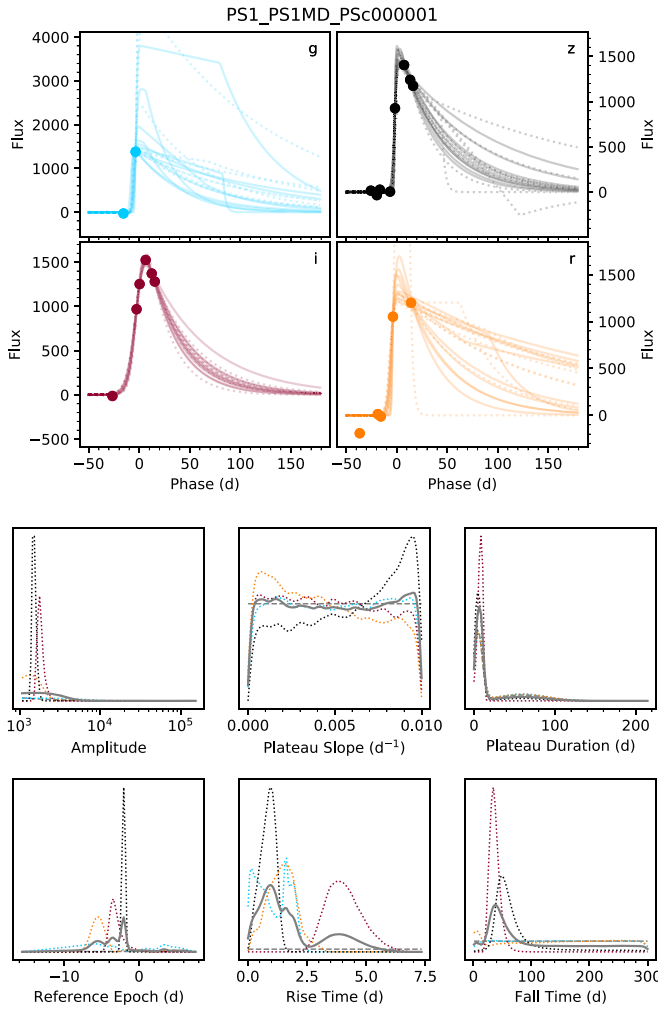
Figure 1. Two-step MCMC fit of Equation (1) to a sample transient. The top panels show the light-curve models in each of the four filters. Dotted lines represent the results of the first iteration, and solid lines represent the results of the second. The bottom panels show how the first-iteration posteriors are combined to produce the second-iteration priors. The gray dashed line is the first-iteration prior, the colored dotted lines represent the first-iteration posteriors for the four filters (same colors as the upper panels), and the gray solid line is the second-iteration prior.
