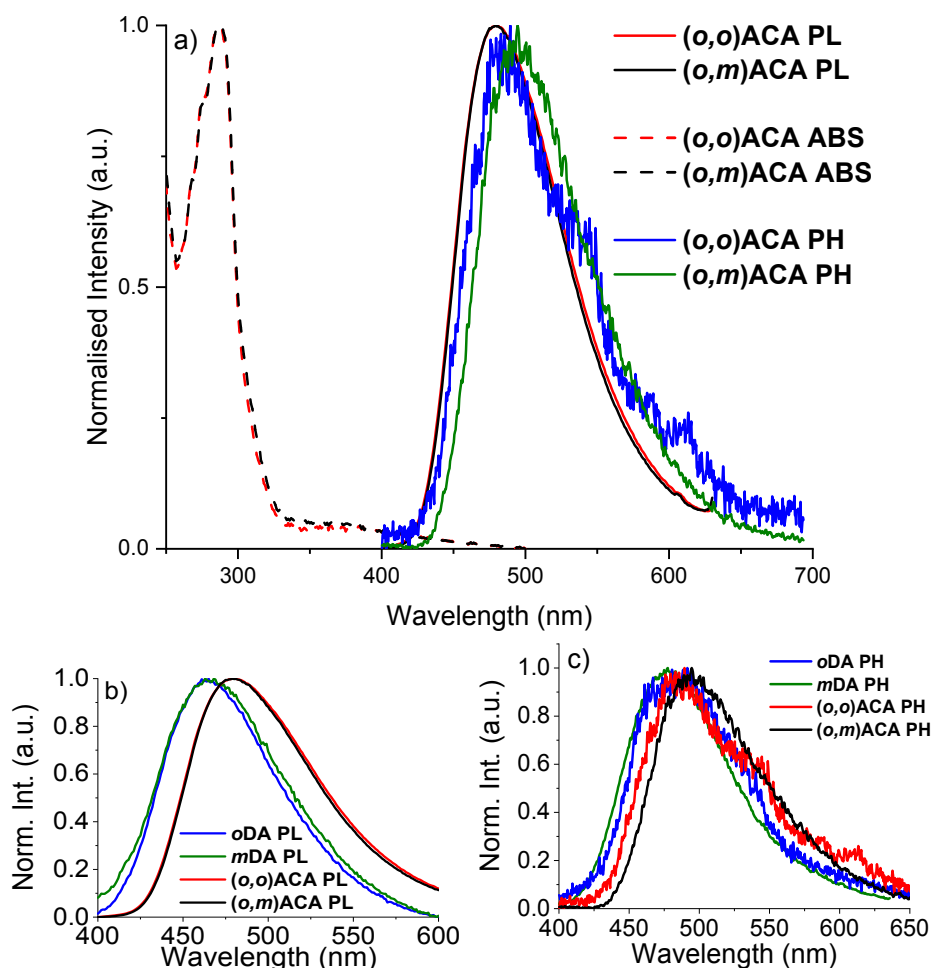
Figure 1: a) Absorption (ABS), photoluminescence (PL) and phosphorescence (PH) spectra of (o,m)ACA and (o,o)ACA in DPEPO films, b) Comparison of PL spectra with previously investigated D-A materials (also in DPEPO host), and c) comparison of PH spectra of the same. PH spectra recorded at >50 ms delay following pulsed 355nm excitation, with sample at 80 K.
