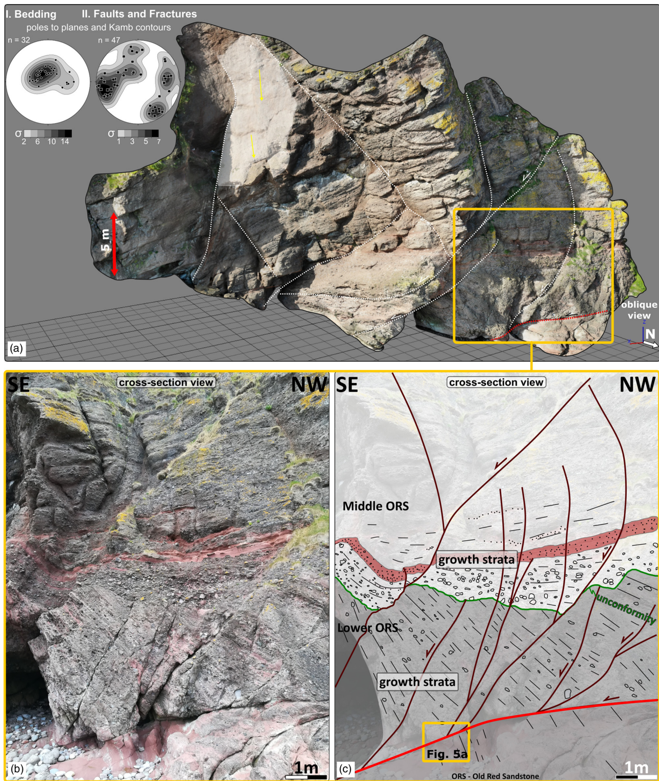
Fig. 4. Cliff exposure below the Nethermill Cottages; location is indicated in Figure 3a . (a) Three-dimensional digital outcrop and inset lower hemisphere equal area stereonets derived from planes extracted from 3D photogrammetric model. Main faults are highlighted in white with senses of offset where known. Lineations on fault plane are shown by yellow lines. Locations of (b) and (c) are indicated by the yellow box. (b) Field photograph and (c) line drawing showing a cross-sectional view looking SW onto the angular unconformity between the Lower and Middle Devonian and main faults with growth strata in their hanging wall. The low-angle fault at the base of the outcrop should be noted. The location of Figure 5a is shown by the yellow box.
