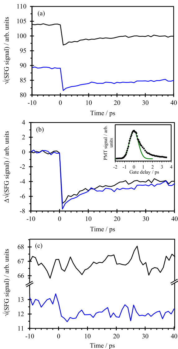
FIG. 2. (a) Transient surface SFG signal (PPP) recorded from aqueous MG without OKG (black) and with OKG (blue). (b) Background-subtracted traces of the same data in (a). The inset shows the efficiency of the Kerr gate as a function of delay between the gate and SFG pulses (dots) with the Gaussian fit (green line). Positive gate delay indicates that the SFG pulse arrives after the gate. (c) Transient surface SFG signal (PPP) recorded from aqueous MG without OKG (black) and with OKG (blue), in the presence of coumarin 2.
