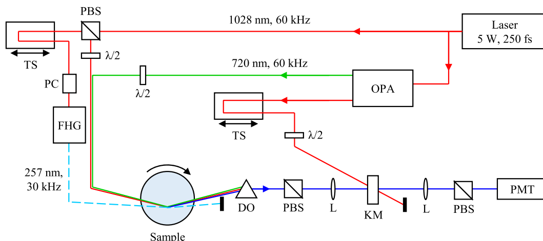
FIG. 1. Simplified schematic of the experimental setup. PBS = polarizing beam splitter, \lambda/2 = half-wave plate, TS = translation stage, PC = Pockels cell, FHG = fourth harmonic generation, DO = dispersing optic (Pellin–Broca prism), L = lens, KM = Kerr medium, and PMT = photo-multiplier tube. Collinear beams are visually offset for clarity.
