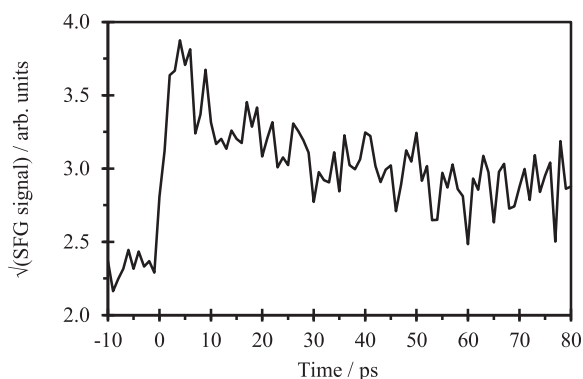
FIG. 3. Transient surface SFG signal (PPP) recorded from 0.1M aqueous sodium phenolate with OKG.
