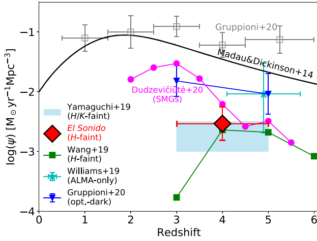
Figure 9. Left: CSFRD contribution of H -faint galaxies presented in this work (red diamonds). CSFRD contribution of H -faint galaxies found by Yamaguchi et al. (2019) and Wang et al. (2019), optical/near-IR-dark galaxies found by Williams et al. (2019) and Gruppioni et al. (2020), as well as AS2UDS SMGs ( S_{870} > 1 mJy; Dudzevičiūtė et al. 2020) are also shown for comparison. The ALMA-based CSFRD evolution measured by Gruppioni et al. (2020) is shown as gray open squares. The analytic model by Madau & Dickinson (2014) is shown as a black solid line. Right: The contribution of H -faint galaxies to the galaxy SMF at z \sim 4 . Unobscured galaxies selected by HST (Song et al. 2016; the blue open circles), VISTA/ K_S (Muzzin et al. 2013; the green open triangles), and K + CH1 (Davidzon et al. 2017; the magenta open squares) are shown for comparison. Black solid line denotes the SMF derived with a semi-analytic model (Behroozi et al. 2019).
