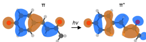
Figure 1. Computed molecular orbitals (MOs) involved in the vertical \pi\pi^* transition of pCK^- that leads to subsequent isomerization on the S_1 excited state (LR-TDDFT/TDA/ \omega B97X-D/ aug-cc-pVDZ).
