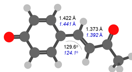
Figure 4. Calculated structure of p\text{CK}^- . The distances and angles between the three bridging carbon atoms connecting the phenyl ring and ketone are indicated for the FC structure (black) and the S_{1,\text{PM}} (blue, italics), obtained at the DFT/ \omega\text{B97X-D/aug-cc-pVDZ} and LR-TDDFT/TDA/ \omega\text{B97X-D/aug-cc-pVDZ} levels of theory, respectively.
