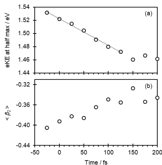
Figure 3. (a) The electron kinetic energy at half maximum of the high energy edge determined from a linear fit, plotted as a function of pump-probe delay. The dashed line is a linear fit to these data. (b) The weighted average of \beta_2 as a function of pump-probe delay.
