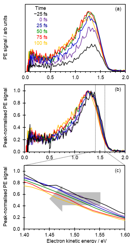
Figure 2. (a) Time-resolved photoelectron spectra of pCK^- following excitation at 2.79 eV and probed at 1.55 eV. (b) Same data as in (a) but with each spectrum normalized to its maximum intensity. (c) Same data as in (b) but focusing on the high kinetic energy edge of the spectra, showing the spectral shift over the first 100 fs.
