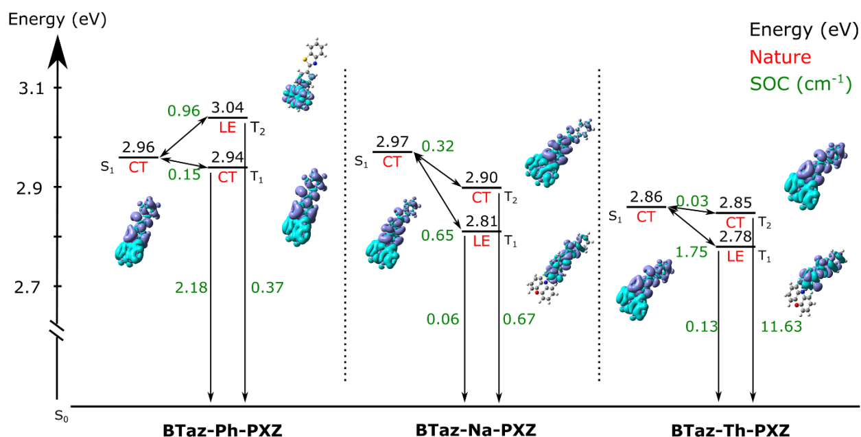
Figure 5. Schematic representation of the ground and excited state energy levels with their corresponding CT/LE character and the spin-orbit coupling values (in \text{cm}^{-1} ) between these various excited states as obtained using TDDFT calculations with LC-BLYP ( \omega = 0.17 \text{ bohr}^{-1} )/6-311G(d) under the TDA and applying the PCM (cyclohexane).
