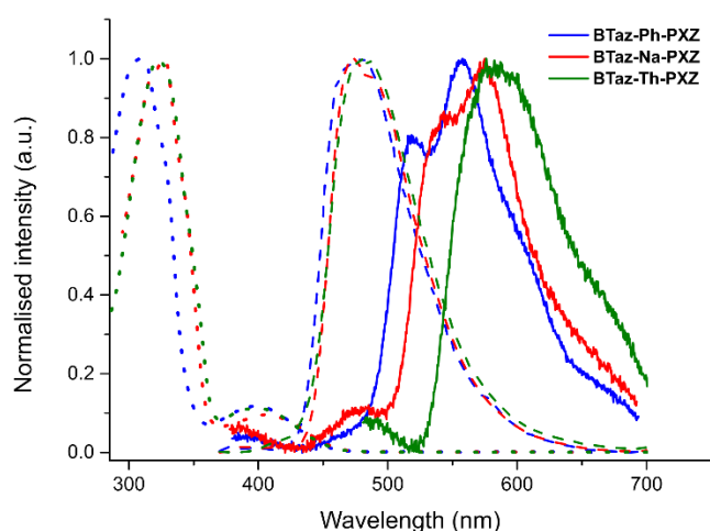
Figure 2. Normalised steady-state absorption spectra in toluene (dotted lines), steady-state emission spectra ( \lambda_{\text{exc}} = 355 nm) at room temperature in zeonex film (dashed lines), and time-resolved phosphorescence ( \lambda_{\text{exc}} = 355 nm) at 80 K at a 44.7 ms decay time in zeonex film (solid lines) for BTaz-Ph-PXZ (blue), BTaz-Na-PXZ (red), and BTaz-Th-PXZ (green).
