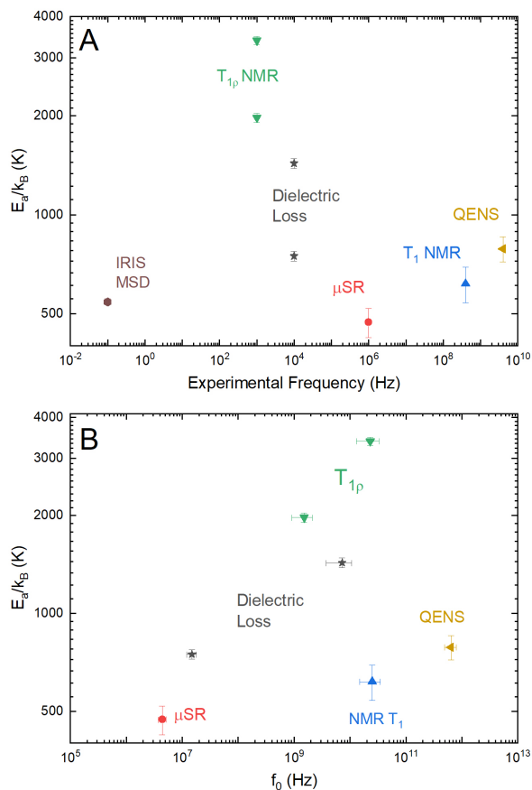
Fig. 7 A: Plot of the fitted activation energy against the experimental frequencies or timescales from different techniques. B: A comparison of the activation energies for each respected technique with their respective attempt frequencies. The values for the dielectric data have been taken from Reference 27 .
