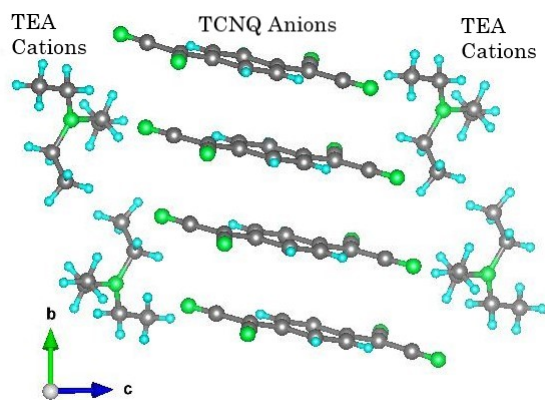
Fig. 1 A view of the structure of the high temperature phase of \text{TEA}(\text{TCNQ})_2 , at T = 298 K, shown along the a -axis, where the C = grey, N = green and H = light blue. Note that the hydrogen positions are an approximation deduced from a Fourier map to give an idea of their different environments, and the ammonium hydrogens (N-H) are not shown as their positions could not be determined. The structure was taken from work within reference 27 .
