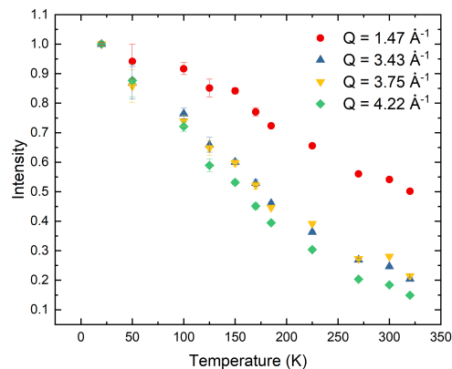
Fig. 4 The temperature variation of the intensity at Q = 4.22, 3.43, 3.75 and 1.47 Å -1 .
