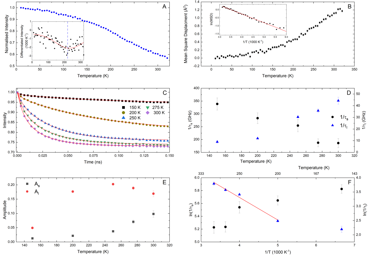
Fig. 5 A: Temperature dependence of the intensity of the QENS peaks performed through an elastic window scan. The inset shows the first derivative of the curve where the blue dashed line is at 220 K and the red curve is a Gaussian where the centre of the peak is at 233(9) K with a FWHM of 203(44) K, illustrating the broadness of the transition. B: The mean square displacement as a function of temperature fit using a Gaussian approximation. The Inset shows the Arrhenius plot of the corresponding MSD data. C: Time dependent spectra where the data has been summed over all of Q , the solid lines are fits to the data. D: The relaxation rates ( \tau_s or \tau_l ) associated with the fits to the data. E: The amplitude of each component from the fits to the data. F: Arrhenius plot of relaxation rates, where the solid line is a fit to the data.
