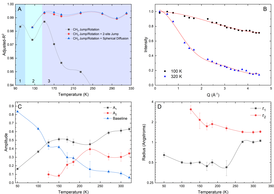
Fig. 3 EISF analysis of the incoherent elastic line scattering from IN13. A: The adjusted R^2 parameters illustrating the quality and applicability of each model to each spectra. The solid lines are purely a guide to the eye. B: Examples of fits (solid red lines) to the I(Q) data at selected temperatures. Equation 1 was fitted to the 50 K C: The temperature dependence of the respective amplitude of each component from the fits to the data. The solid lines are guides to the eye. D: The radius associated with the two component fits to the data where r_1 is for the \text{CH}_3 jump rotation and r_2 is for the spherical diffusion model. The solid lines are guides to the eye.
