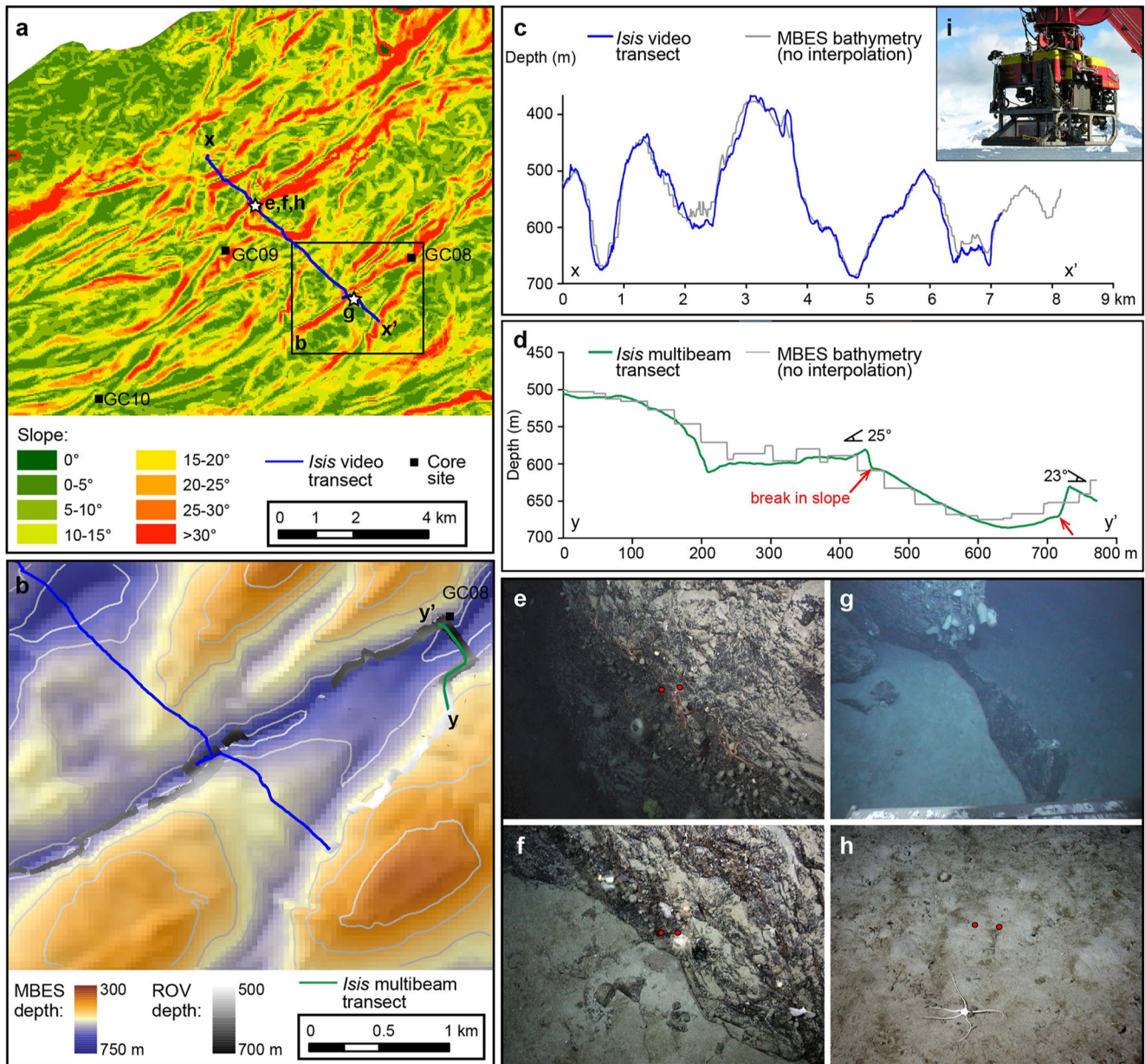
Figure 2. Detailed marine observations of the inner shelf channel system. (a) First derivative of bathymetry, slope, over the channels (same area as Figure 1b). (b) Location of remotely operated vehicle (ROV) video survey line and multibeam surveys near the GC08 core site (located in Figures 1b and 2a). (c and d) Comparison of seafloor profiles from shipborne MBES and ROV bathymetry over bedrock channels (located in 2a, 2b). (e–h) ROV bottom photographs (e, f, h) and video stills (g) showing the character of the seafloor in the bedrock channel system. The red circles in (e, f, h) are 10 cm apart; the frame in (g) is about 1 m wide (photos are located in 2a). (i) Isis ROV being deployed during JR157.
