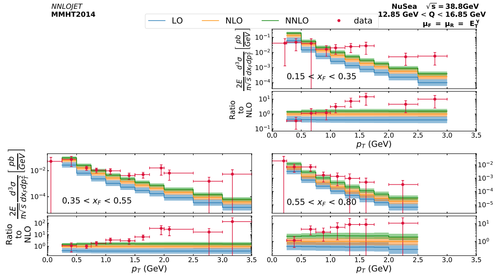
Fig. 9. Transverse momentum distribution of lepton pairs with 12.85 \text{ GeV} < Q < 16.85 \text{ GeV} in different bins in x_F , compared to data from the NuSea experiment [27,28].
