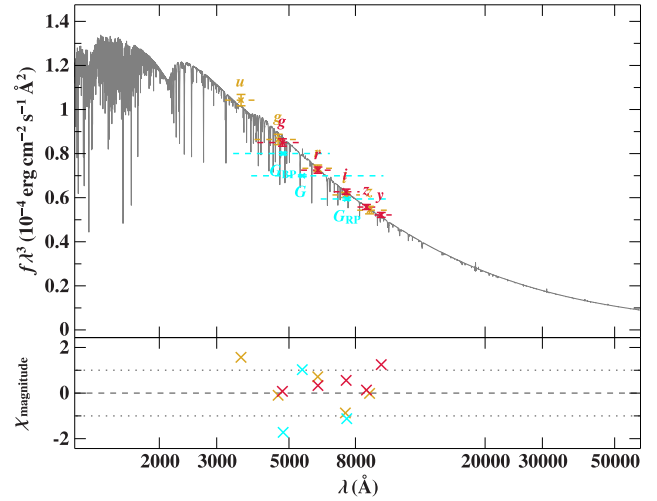
Figure B3. SED fit for J1603+3412 using SDSS (ochre; Alam et al. 2015), Pan-STARRS (dark red; Magnier et al. 2020), and Gaia EDR3 (cyan; Riello et al. 2021).
