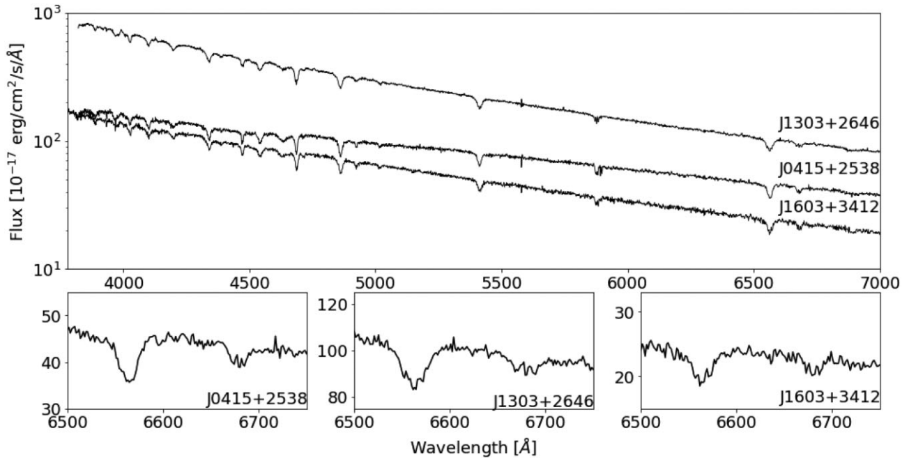
Figure 1. SDSS spectra of J0415+2538, J1303+2646, and J1603+3412 are shown in the top panel. The bottom panels zoom in the region around H\alpha and the He I 6678 Å line, which show hints of Zeeman splitting. J0415 + 2538 is in a region with strong reddening (see Section 3.1).
