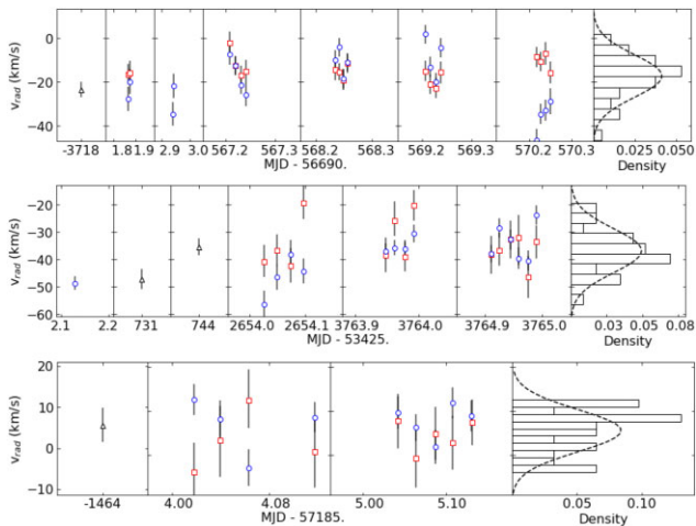
Figure 4. Radial velocities for J0415+2538, J1303+2646, and J1603+3412, from top to bottom. Estimates obtained from the red and blue WHT arms are shown as red squares and blue circles. Estimates from the SDSS spectra (two available in the case of J1303+2646) are shown as black triangles. The right-hand-most panel shows a histogram of the values, with a normal distribution with mean and standard deviation derived from the measurements for comparison.
