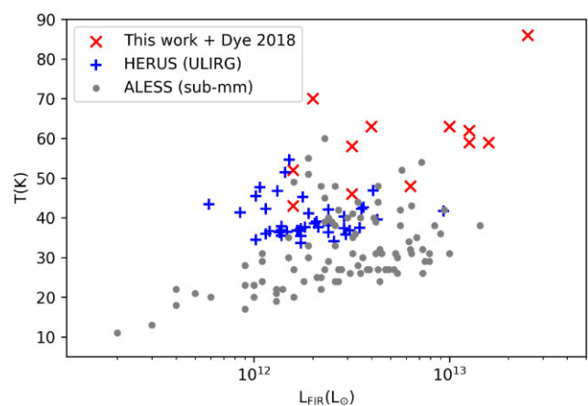
Figure 4. Temperature distribution as a function of far-IR luminosity. The red crosses show the luminosities taken from this work (excluding HeLMS J235331.9+031718), and Dye et al. (2018). The spectroscopic redshift range of this combined dataset is approximately z \sim 1-4 . The blue pluses show the data taken from the HERUS Survey (Clements et al. 2017), with a spectroscopic redshift range of approximately z \sim 0.02-0.26 . The grey dots come from the ALESS survey (Swinbank et al. 2013), with a photometric redshift range of z \sim 0.5-6.5 .
