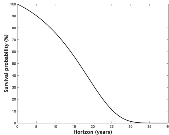
Figure 5. Survival probabilities for Australian males just turned age 70. Notes: See Figure 4 caption. For an individual aged x = 70 , the survival probabilities are p(s) = p(s - 1)(1 - q(s)) where p(0) = 1 and s = 1, \dots, 40 .
