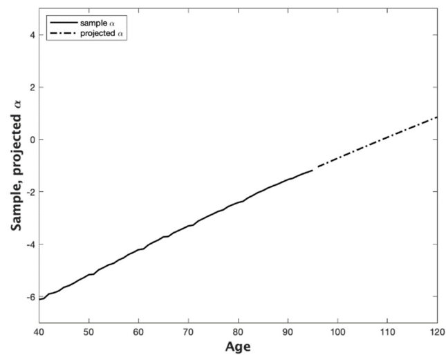
Figure 3. Australian males fitted age effect, \hat{\alpha} , and projected age effect, \alpha : Ages 40 to 120. Notes: Based on the CBDX3 model applied to Australian male deaths and exposures data for sample years 1921–2014 and sample ages 40–95. Source: Human Mortality Database.
