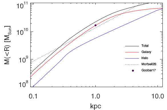
Fig. 9. Circularly averaged integrated mass profiles of the best model for the case where only positional constraints are used. The profile of the galaxy is shown in red and the profile of the halo is shown in blue. The profile of the total mass is shown as a black curve. The black dot at 1 kpc is the estimated mass in the original lens model of Goobar et al. (2017). The dotted line is the new estimate by Mörtzell et al. (2020) using a circular aperture. An isothermal profile scales its integrated mass as the radius.
