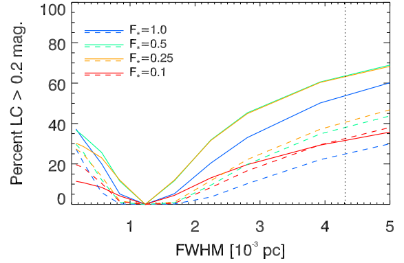
Fig. 19. Same as Fig. 18 but for images 3 (solid lines) and 4 (dashed lines).
