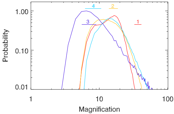
Fig. B.1. Marginalized probability distribution of the magnification for the case \alpha = 0.8 . Only the four positions of the SNe images are used as constraints. The curves show the marginalized probability for each of the four SNe images. The horizontal colored lines show the inferred range of magnification from observations.
