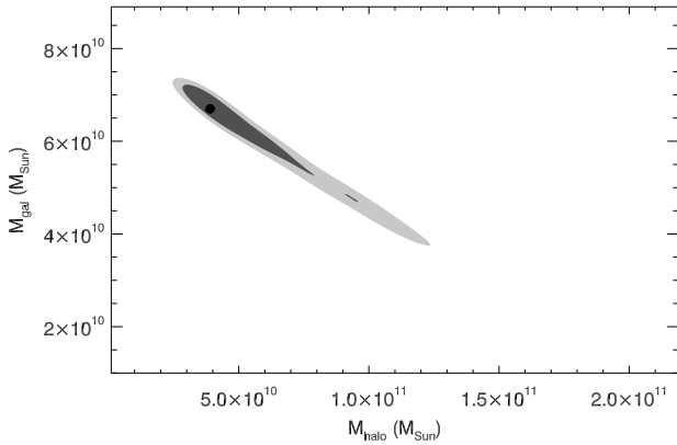
Fig. 12. Marginalized probability in the M_{\text{halo}} - M_{\text{gal}} plane.
