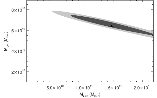
Fig. B.7. Marginalized probability in the M_{\text{halo}}-M_{\text{gal}} plane for the case \alpha = 1.4 . The best model is marked with a black dot and has a likelihood value of \ln(\mathcal{L}) = 0.1871 .
