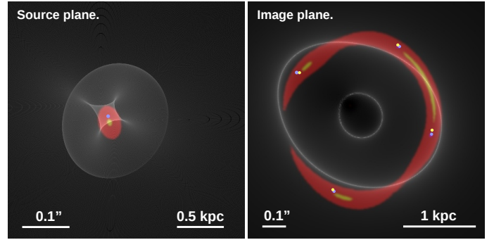
Fig. 7. Caustics (left) and critical curves (right) for the model where only position is used. A simple source with just three components, nucleus (orange), halo (red) and SN (blue) is shown in the left panel (source plane). The predicted image is shown in the right panel (image plane). The yellow dots in the right panel mark the observed position of the four SN images.
