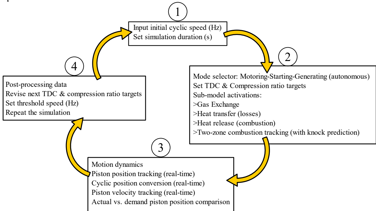
Fig. 5. Schematic of real-time interaction model implementation Model schematic.
