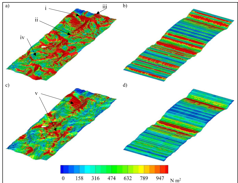
Figure 7. The total Reynolds stresses on the bed calculated, for (a and b) Primary Reynolds stress ( \sum -\rho u'w' ) and (c and d) secondary Reynolds stress ( \sum -\rho v'w' ) for the (a and c) 3D and (b and d) 2D topography.
