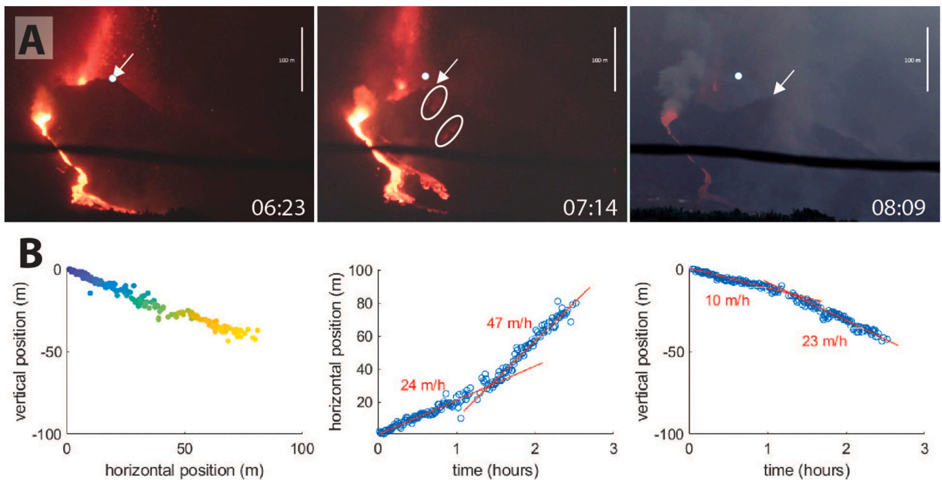
Fig. 4. Kinematic observations of the proximal block rafting. A: Still frames from a video collected from Finca La Cruz (Tazacorte), ~7 km. from the vent. White dot and arrow mark a reference point and its displacement over time. Dashed ovals encircle landslides on the collapsing flank of the cone. Scale bar is 100 m long at the vent. B: Manual tracking of the point indicated by the arrow in the upper panel. Left-hand panel: over the whole video the point moved almost linearly 81 m westward (right) and 42 m downwards (apparent displacement, projected on a plane perpendicular to the line of sight). The colour key shows increasing time from blue to yellow. Middle- and right-hand panels: The horizontal and vertical apparent displacement of the tracked point over time. (For interpretation of the references to colour in this figure legend, the reader is referred to the web version of this article.)
