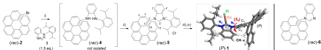
Scheme 1. Left: Synthesis of enantiopure helicene-NHC-Cu complex ( P )- and ( M )-1. i ) Pd(OAc) 2 (10 mol%), Xantphos (10 mol%), Cs 2 CO 3 (3 eq.), dry toluene, MW, 170 ° C, 30 min; ii ) conc. HCl, (EtO) 3 CH, 85 ° C, overnight (58%, two steps); iii ) CuCl (1.2 eq.), K 2 CO 3 (3 eq.), acetone, 60 ° C, overnight, 49%; iv ) chiral HPLC (( S,S )-Whelk-O1). X-ray diffraction structure of ( P )-1 with highlighted additional ( S a ) axial chirality observed in the solid state. Right: Structure of the [6]helicene-2- N -benzimidazole system 6 ; for its synthetic details see Reference 10e.
