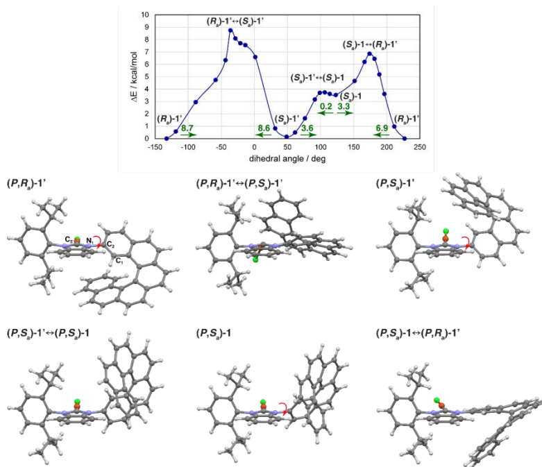
Figure 3. Energy profile for the rotation around N_1(\text{NHC})-C_2(\text{helicene}) bond in the helicene-NHC-Cu complex 1 (top, to increase legibility, helicene stereochemistry designation ( P ) has been omitted in the structures' labels) along with molecular structures corresponding to its characteristic points (bottom). Numbers listed along arrows displayed in the chart are estimated energy barriers (in kcal/mol) of the transition between two adjacent minima in the direction indicated by the arrow. Based on TPSS+D3/TZVP calculations with continuum solvent model for dichloromethane.
