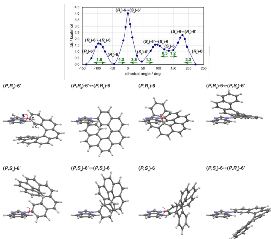
Figure 4. Energy profile for the rotation around N_1(\text{imidazole})-C_2(\text{helicene}) bond in the helicene-benzimidazole ligand 6 (top, to increase legibility, helicene stereochemistry designation ( P ) has been omitted in the structures' labels) along with molecular structures corresponding to its characteristic points (bottom). Numbers listed along arrows displayed in the chart are estimated energy barriers (in kcal/mol) of the transition between two adjacent minima in the direction indicated by the arrow. Based on TPSS+D3/TZVP calculations with continuum solvent model for dichloromethane.
