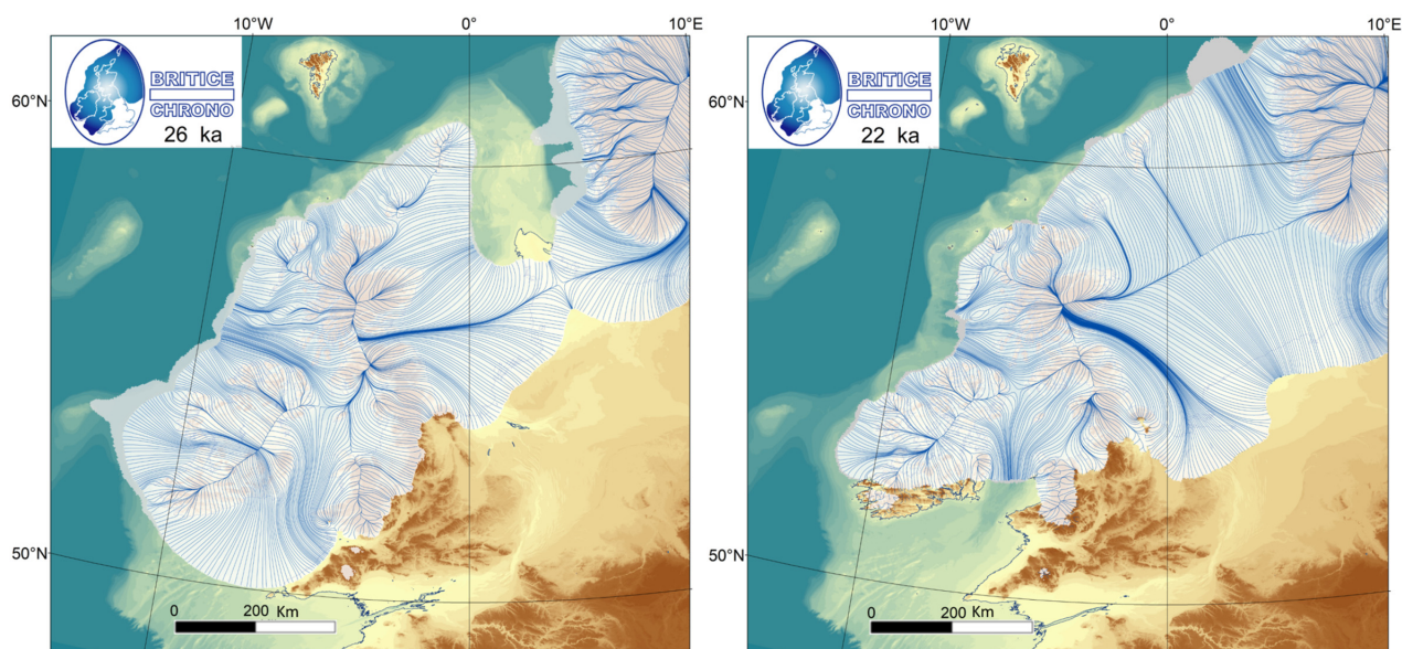
Fig. 7. Ice-sheet extent and flow geometry (ice shelves in grey) at the maximum areal extent of the British–Irish Ice Sheet (left panel; 26 ka) and North Sea Ice Sheet (right panel; 22 ka). Build-up of ice over the North Sea occurred by head-on collision of British and Scandinavian ice lobes (left panel; 26 ka) resulting in an ice saddle that rapidly grew in elevation to build the major North Sea Ice Divide (1500 m thick) by 22 ka.
