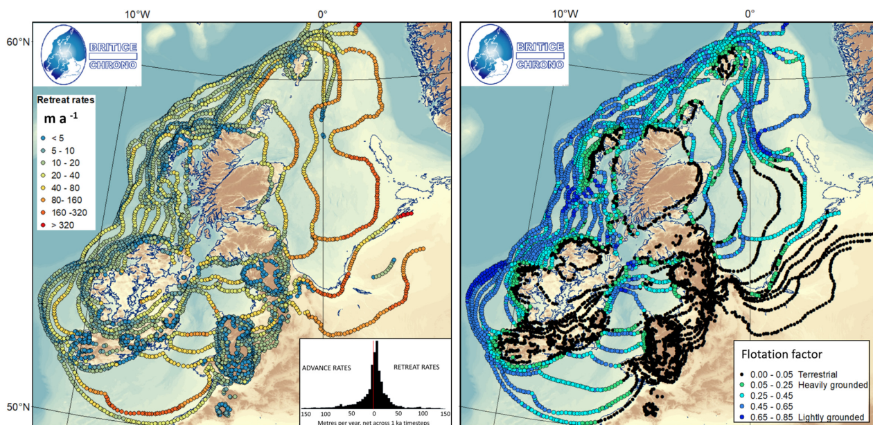
Fig. 13. Left panel: net rates of retreat calculated at 1-ka timesteps, demonstrating large variations between terrestrial ( 50 \text{ m a}^{-1} ) and marine sectors ( >50 and up to 451 \text{ m a}^{-1} ). Note that these time-averaged values likely mask faster shorter-lived rates that are below our dating resolution. Inset panel shows frequency distribution of rates of retreat and advance. Right panel: flotation factor for marine-terminating margins (advancing and retreating) calculated using ice thickness behind grounding lines and water depths from the relative sea level modelling (black indicates terrestrial-terminating ice margins). Comparing both maps indicates a general correspondence between faster retreat for margins that were marine-based and for those that were more lightly grounded (high flotation factors).
