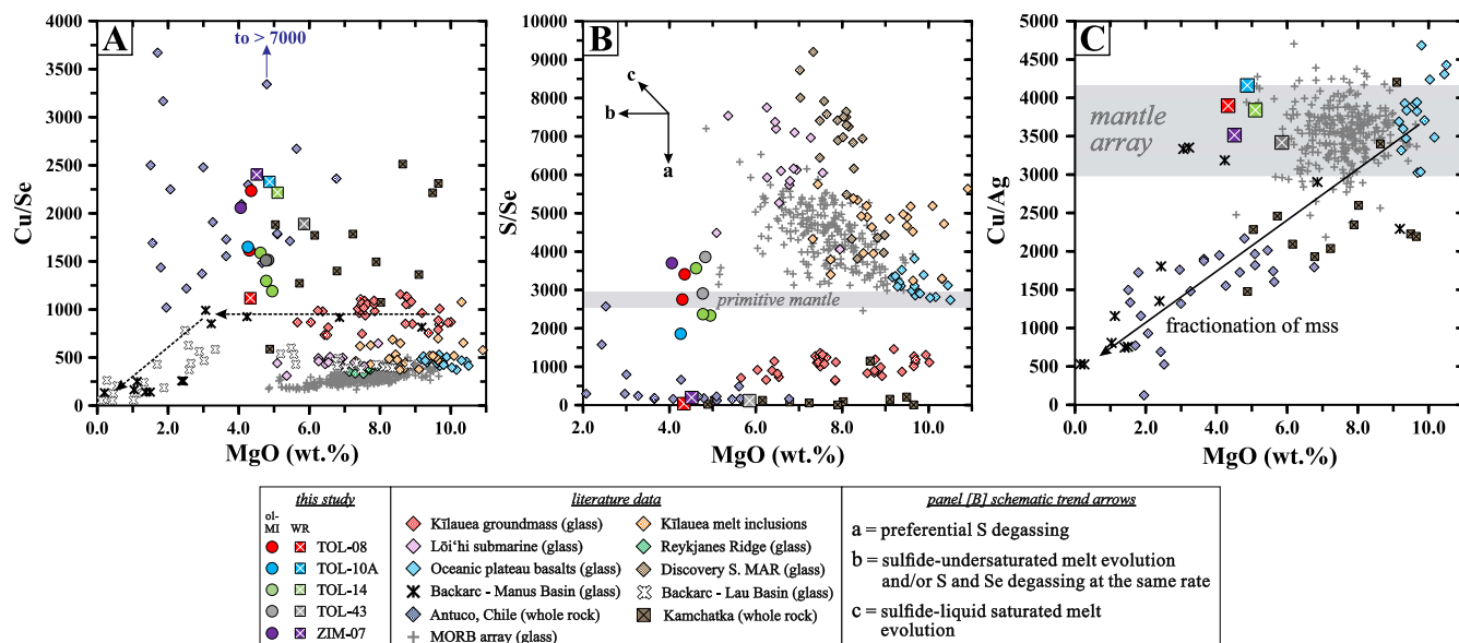
Fig. 9. Chalcophile element trends as a function of MgO (wt.%) in the melt inclusions and bulk rocks of this study along with available literature data for melt inclusions, groundmass glasses, and bulk rocks from other Kamchatka volcanoes and other tectonic settings. [A] Cu/Se ratios; [B] S/Se ratios; [C] Cu/Ag ratios. Schematic arrows apply to panel [B] only and illustrate the broad trends expected by each process on a given data set. Data sources for literature samples included for comparison are as follows: Kilauea and Loi'hi glasses (Wieser et al. , 2020); Reykjanes Ridge (Jenner et al. , 2012); Oceanic plateau basalts (Reekie et al. , 2019); discovery southern Mid-Atlantic ridge (Lissner et al. , 2014); Manus and Lau backarc basin samples (Jenner et al. , 2012, 2015); MORB array (Jenner & O'Neill, 2012; Reekie et al. , 2019); Kamchatka (Iveson et al. , 2021); Antuco (Cox et al. , 2019). Primitive mantle S/Se value taken from Palme & O'Neill (2014). Note that two bulk rock Tolbachik samples are not shown in panel [B] due to S concentrations below detection limit.
