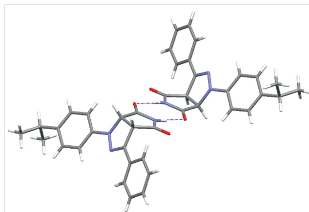
Figure 2 Crystal structure of 6d displaying strong intermolecular H-bonding (CCDC-2221468)
