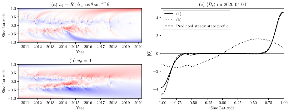
Fig. 3 Effect of meridional flow in the simulation from Fig. 1, showing latitude-time plots of \langle B_r \rangle when the flow is included (a) or omitted (b). Panel (c) shows the latitudinal profiles of \langle B_r \rangle at the end of the simulation. The dashed curve shows the (near) steady-state profile (11) for the case with flow. (After Fig. 3 of Sheeley 2005)
