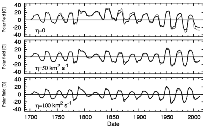
Fig. 10 Application of the radial diffusion term to reduce spurious cycle-to-cycle memory in the SFT model, from Baumann et al. (2006). The top row shows the north polar field (above 75° latitude) in a simulation with no radial diffusion, while the middle and bottom rows show the same simulation with \eta_0 = 50 \text{ km}^2 \text{ s}^{-1} and 100 \text{ km}^2 \text{ s}^{-1} according to the prescription in Sect. 5.2. The simulation uses random emerging BMRs proportional to the observed sunspot numbers. The dashed line shows a simulation started in 1750, illustrating how the memory of the initial conditions persists. (© ESO. Reproduced with permission.)
