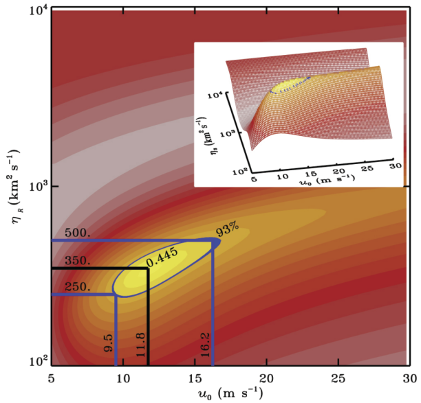
Fig. 4 Fitness function \chi^{-2} as a function of meridional flow amplitude u_0 = \max_{\theta} |u_{\theta}| (horizontal axis) and diffusivity \eta_R \equiv \eta (vertical axis), from the optimization study of Lemerle et al. (2015). Black lines show the optimum value and blue lines the limit of the acceptable region ( \chi^{-2} \geq 93\% \chi_{\max}^{-2} ). (© AAS. Reproduced with permission.)
