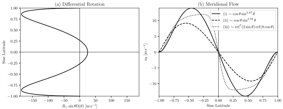
Fig. 2 Velocity profile of differential rotation in the Carrington frame (a), and some example optimized profiles of meridional flow velocity (b), including (i) the simulation shown in Fig. 1; (ii) the Cycle 21 simulation of Whitbread et al. (2017); and (iii) the Cycle 21 simulation of Lemerle et al. (2015). The corresponding values of \Delta u are (i) 0.7 \times 10^{-7} \text{ s}^{-1} , (ii) 0.4 \times 10^{-7} \text{ s}^{-1} , and (iii) 1.6 \times 10^{-7} \text{ s}^{-1}
