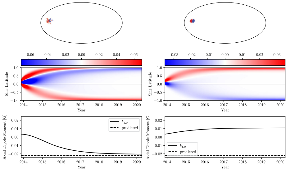
Fig. 8 Evolution of an active region with asymmetric bipolar shape, taken from the simulation in Fig. 1. The left column shows the region with its observed shape, with second row showing \langle B_r \rangle and third row the axial dipole strength b_{1,0} . The right column shows the evolution of an “equivalent” symmetric BMR having the same initial flux and b_{1,0} . The dashed line shows the final b_{1,0} predicted by equation (36) using the observed magnetogram
