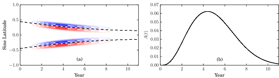
Fig. 9 The smooth source term \langle S \rangle(\lambda, t) used by Petrovay and Talafha (2019). In (a), red/blue contours show \langle S \rangle , and dashed lines indicate \pm \sin[\lambda_0(t)] from (39). Panel (b) shows the overall cycle shape A(t) from (38) with a = 0.00185 , b = 4.058 , c = 0.71
