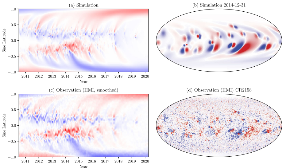
Fig. 1 An SFT model for Solar Cycle 24 with emerging regions derived from SDO/HMI SHARPs data (following the method of Yeates 2020). Panel (a) shows the longitude-averaged field \langle B_r \rangle in the simulation, and (b) shows a snapshot of the two-dimensional field B_r on 31 December 2014. For comparison, (c) shows a magnetic butterfly diagram (or super-synoptic map) constructed from SDO/HMI pole-corrected synoptic maps (Sun 2018), smoothed to a comparable resolution to the simulation. The individual, unsmoothed synoptic map for Carrington rotation CR2158 is shown in (d). Red/blue denote positive/negative values, capped at \pm 10 G in (a,c) and \pm 50 G in (b,d)
