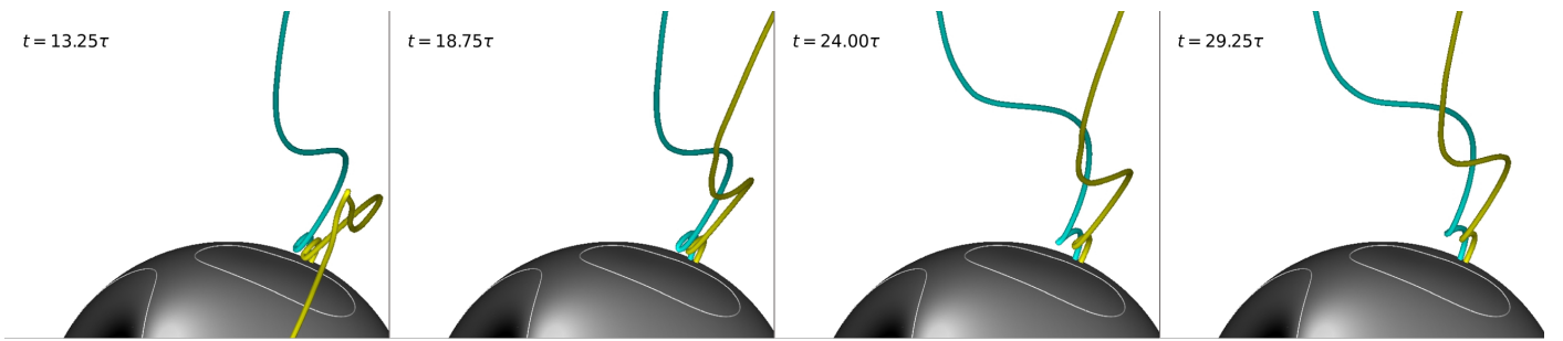
Fig. 13. Temporal evolution of the field lines n°16 (cyan) and 20 (yellow). An animation of this picture is available online showing such apparent slipping motion for both lines.
