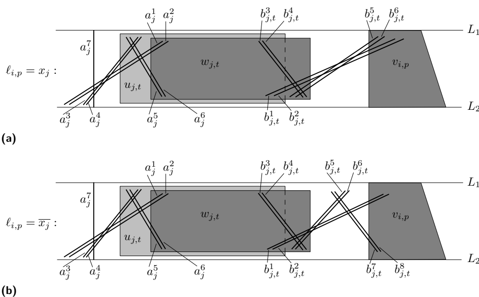
■ Figure 7 The composition of the trapezoids of R_{x_j} with the trapezoid v_{i,p} of R_{\alpha_i} , in the cases where (a) \ell_{i,p} = x_j and (b) \ell_{i,p} = \overline{x_j} .
