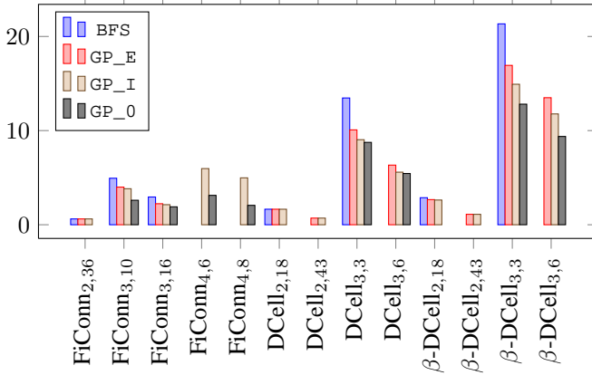
Fig. 2. Percent mean hop-length savings over DR.
