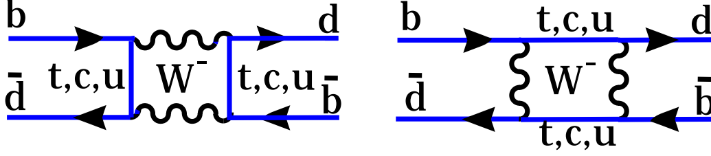
Figure 1: Box diagrams triggering the transition of a \overline{B}_d -meson into a B_d meson.
