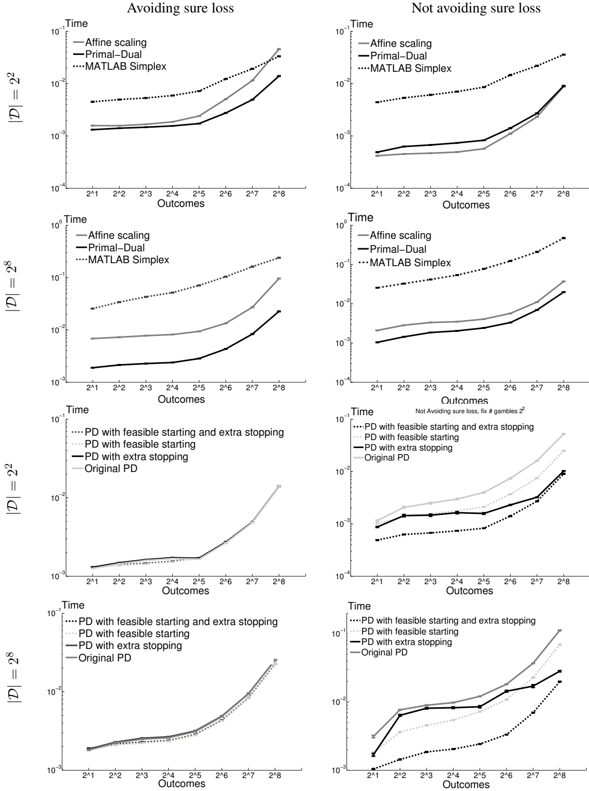
Figure 1: Comparison plots of the average computational time for three methods and for different improved primal-dual methods (PD).
