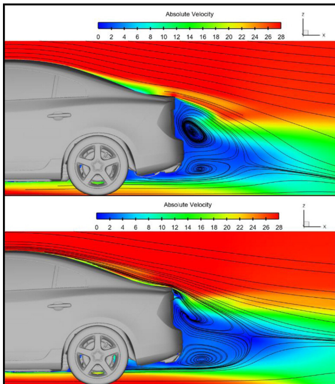
Figure 19. Absolute velocity contours with streamlines for full scale Volvo S60 (2010MY), for y_3 = -80 mm and y_4 = -120 mm planes.
