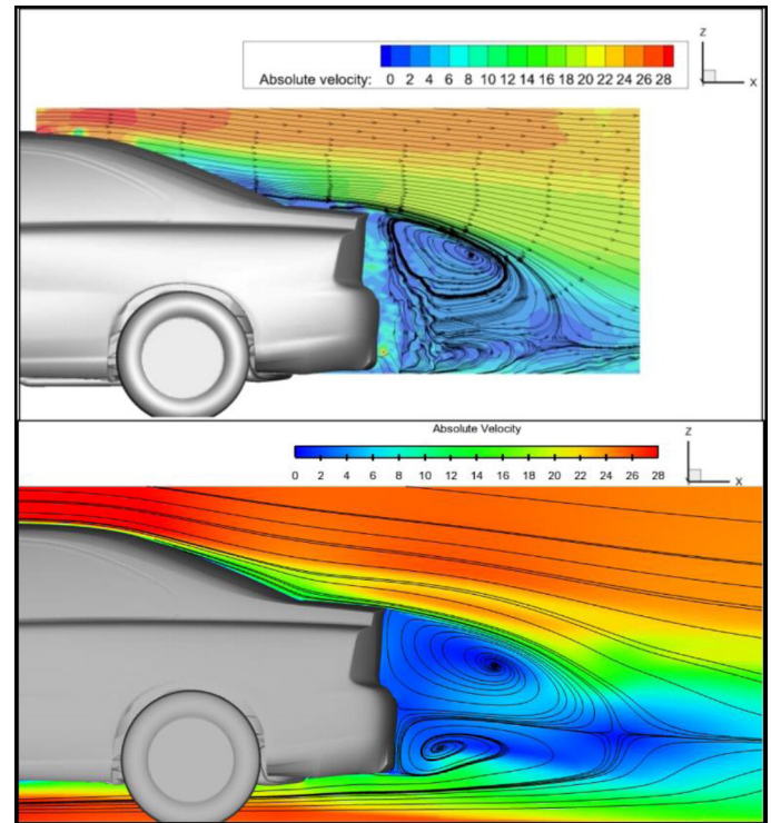
Figure 15. Absolute velocity contours with streamlines for y_3 = -80 mm.
