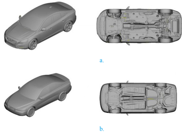
Figure 5. Numerical models with open cooling and detailed underbody (a) 2010MY Volvo S60, (b) 2003MY 30% Volvo S60.
