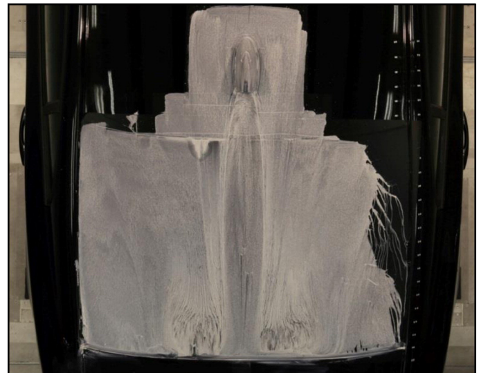
Figure 11. (a) Limiting streamline pattern over the rear window of a full scale car, (b) with reduced amount of paint in the area of separation bubbles, (c) graphical interpretation of the limiting streamline pattern.
