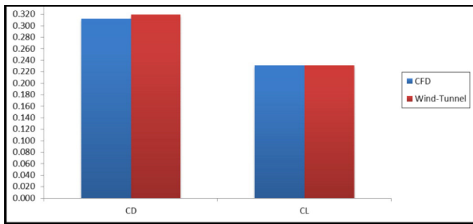
Figure 23. Force coefficients comparison for the 30% scale model Volvo S60 [2003MY] without the antenna for both CFD and 2m 2 wind-tunnel.
