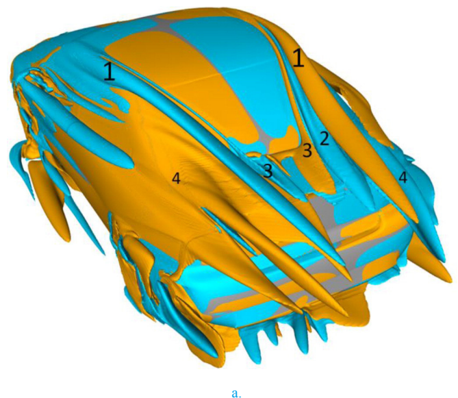
Figure 20. X-component vorticity ( \pm 250 ) in (a) Isometric view, (b) Rear view for the 30% scale model Volvo S60.
