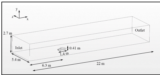
Figure 6. Numerical wind tunnel with relative vehicle position.
