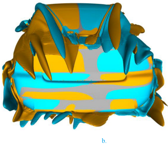
Figure 20. (cont.) X-component vorticity ( \pm 250 ) in (a) Isometric view, (b) Rear view for the 30% scale model Volvo S60.
