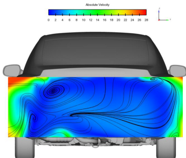
Figure 16. YZ absolute velocity contours with streamlines for x = 1757 mm.
