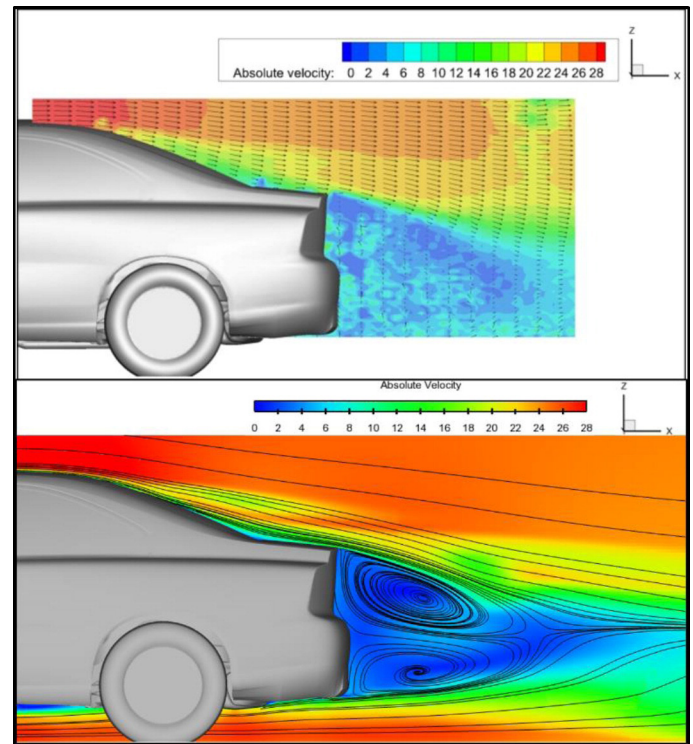
Figure 17. Absolute velocity contours with streamlines for y_4 = -120 mm.
