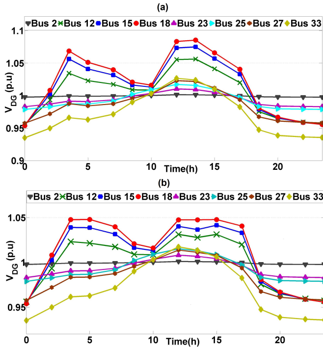
Fig. 4. DGs bus voltage level (a) without control action (b) with coordinated control action.
