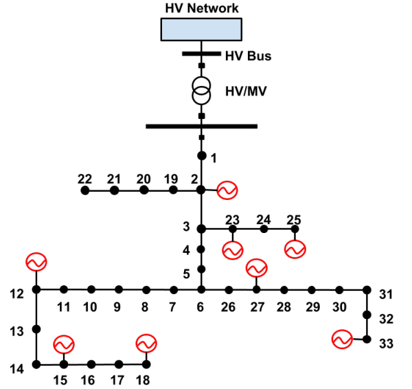
Fig. 2. Radial 33-bus DN under test.
