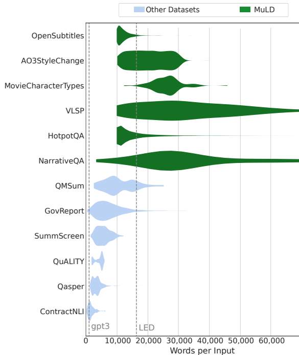
Figure 1: Comparison of lengths of multitask long document benchmarks. The maximum input length of gpt3 and Longformer (LED) are included for comparison.
